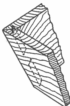
BEVELED MITER JOINT
