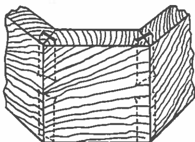
ANGLE JOINT
