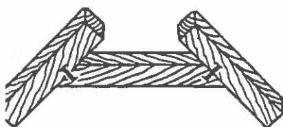
BRACED CORNER JOINT
