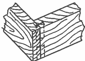
CORNER BUTT JOINT
