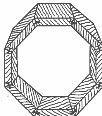
OCTAGON ANGLE JOINT
